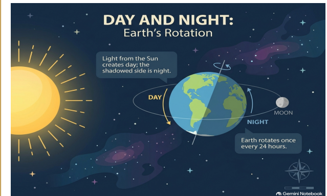
Earth & Space Solar System Orbits
